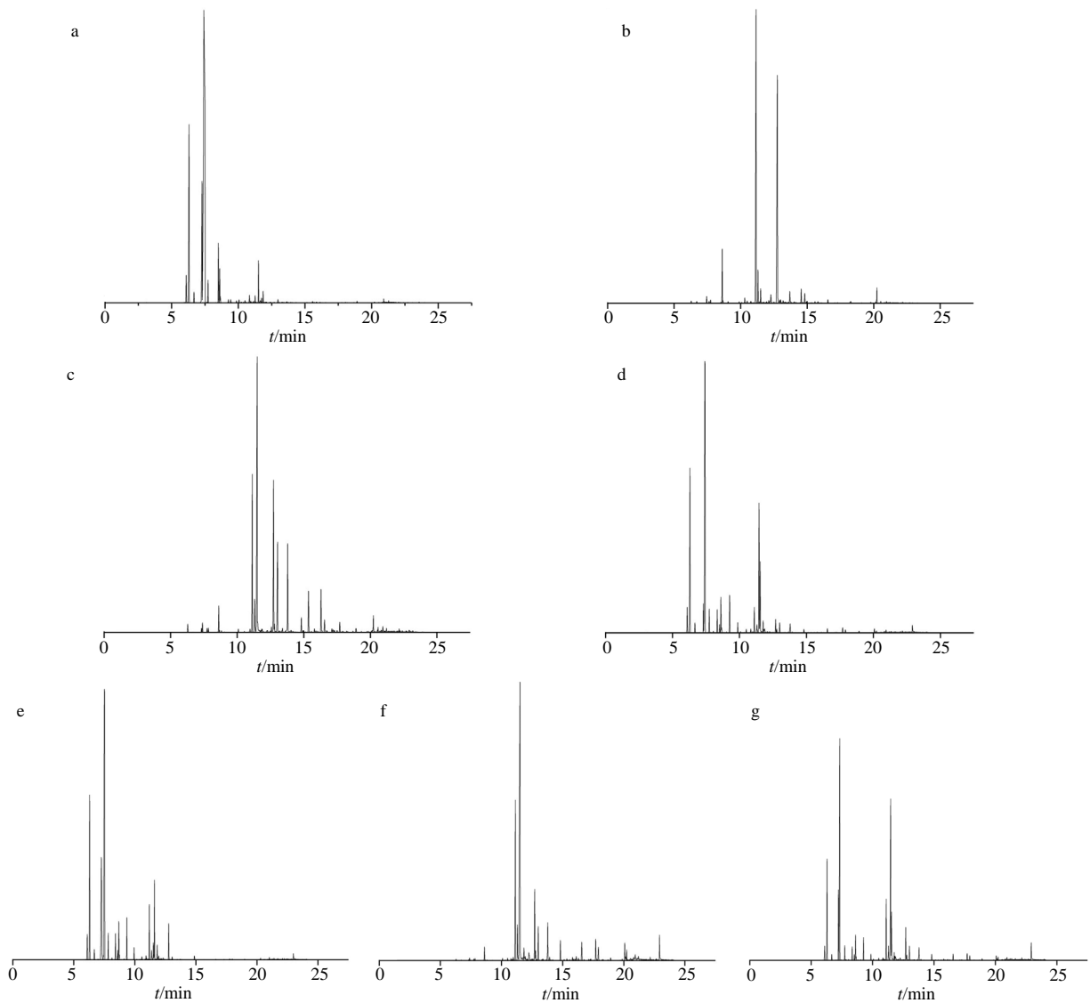
a-连翘挥发油 b-荆芥挥发油 c-薄荷挥发油 d-连翘-荆芥挥发油 e-连翘-薄荷挥发油 f-荆芥-薄荷挥发油 g-连翘-荆芥-薄荷挥发油 a-volatile oil of Forsythiae Fructus b-volatile oil of Schizonopetae Herba c-volatile oil of Menthae Haplocalycis Herba d-volatile oil of Forsythiae Fructus and Schizonopetae Herba e-volatile oil of Forsythiae Fructus and Menthae Haplocalycis Herba f-volatile oil of Schizonopetae Herba and Menthae Haplocalycis Herba g-volatile oil of Forsythiae Fructus , Schizonopetae Herba , and Menthae Haplocalycis Herba
