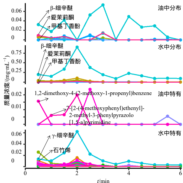
圆点代表不同的化合物,线条表示相应化合物的时间-含量曲线 Cycles indicate different compounds, lines indicate time-content curve of corresponding compound
